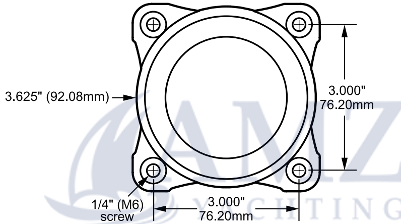
E-Series Battery Switch Dimensions
